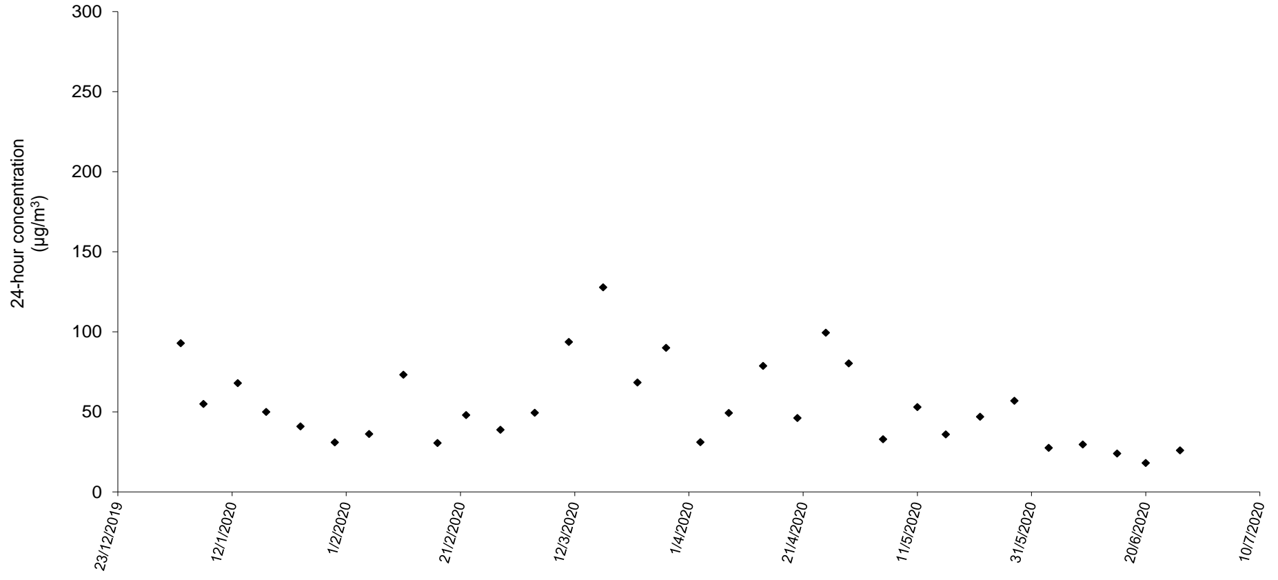
24-hour TSP concentration vs date for Location W-A6
